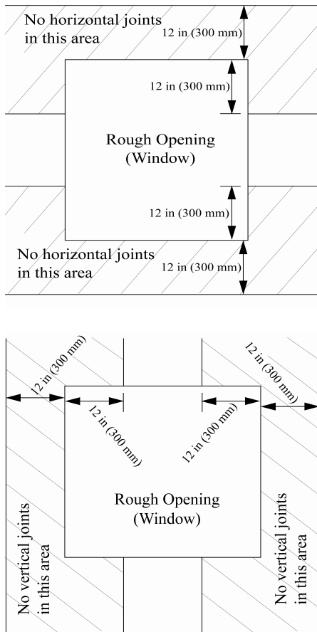
Figure 3 Typical joint locations at window openings
