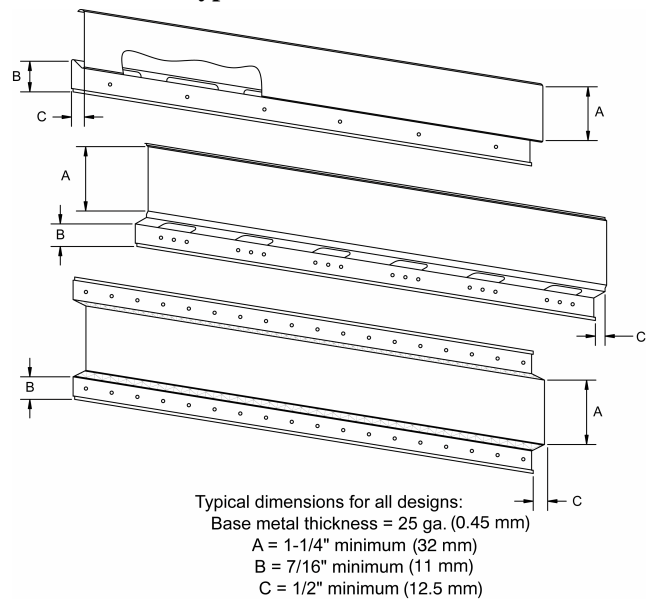
Figure 1 Typical resilient channels
