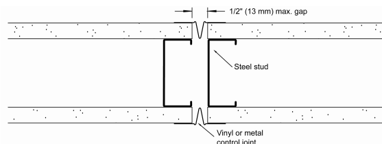
Figure 4 Typical control joint
