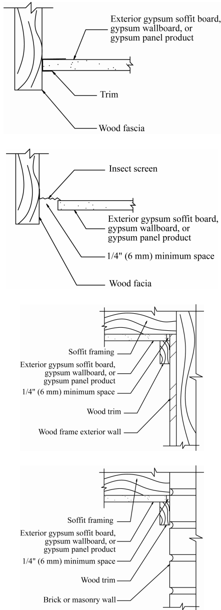
Figure 18 Typical soffit details
