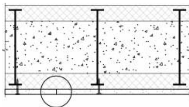
Figure 12 Typical gypsum panel vertical joint location relative to Insulating Concrete Form cross ties
