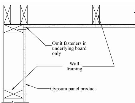
Figure 7 Horizontal section through interior vertical angle
