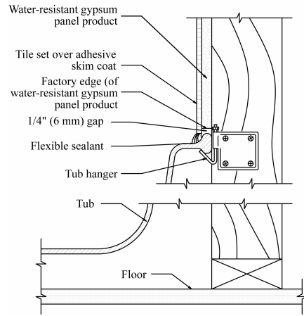
Figure 16 Typical details – shower pan installation
