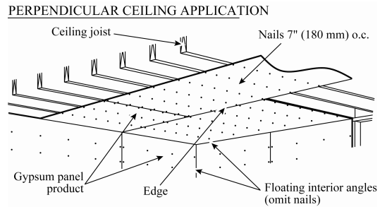
Figure 8 Single nailing
