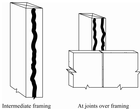
Figure 10 Adhesive application patterns
