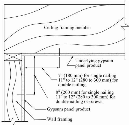
Figure 6 Vertical section, ceiling framing oriented parallel to wall
