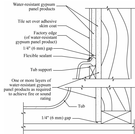
Figure 17 Typical details – tub installation in fire-rated or sound-rated system
