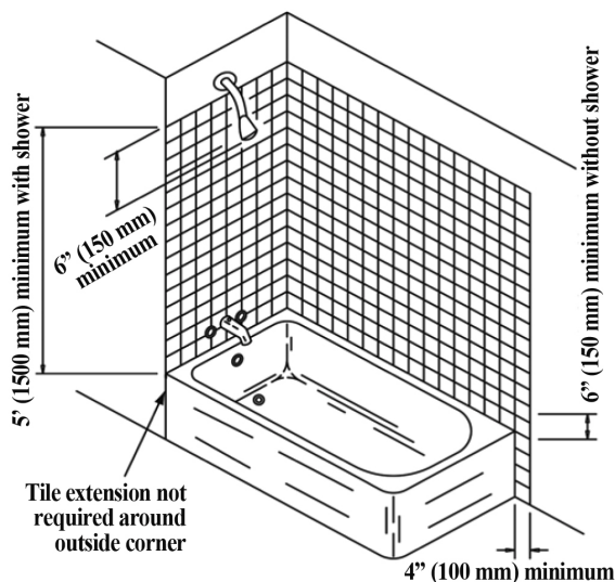
Figure 19 Tile in bath and shower should be brought up to the levels shown.
