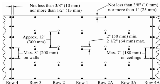
Figure 9 Double nailing
