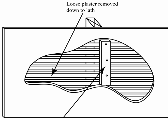
Figure 13 Shimmed plaster wall
