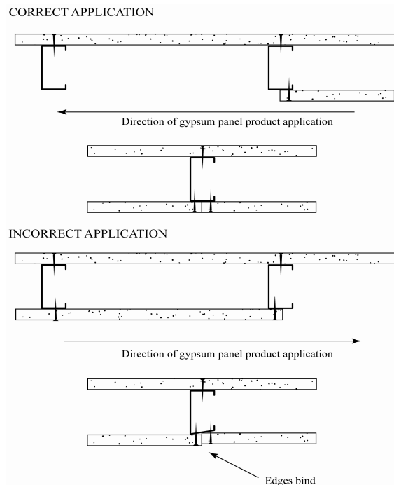
Figure 11 Direction of gypsum panel product application to steel framing
